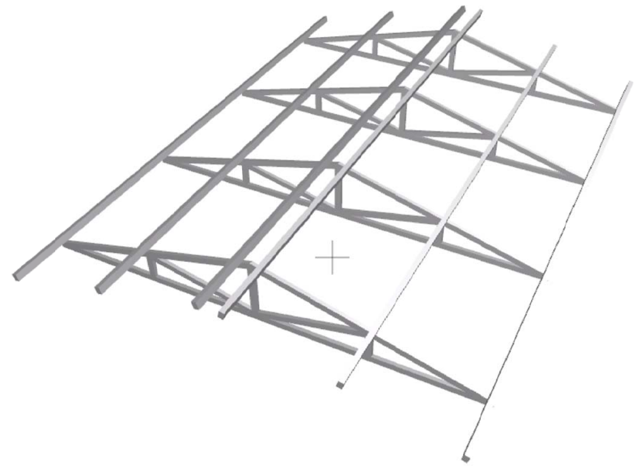
roof structure 3d view
